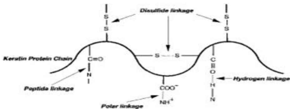
Fig. 1: Simplistic presentation of chemical bonds involved in a nail keratin chain
